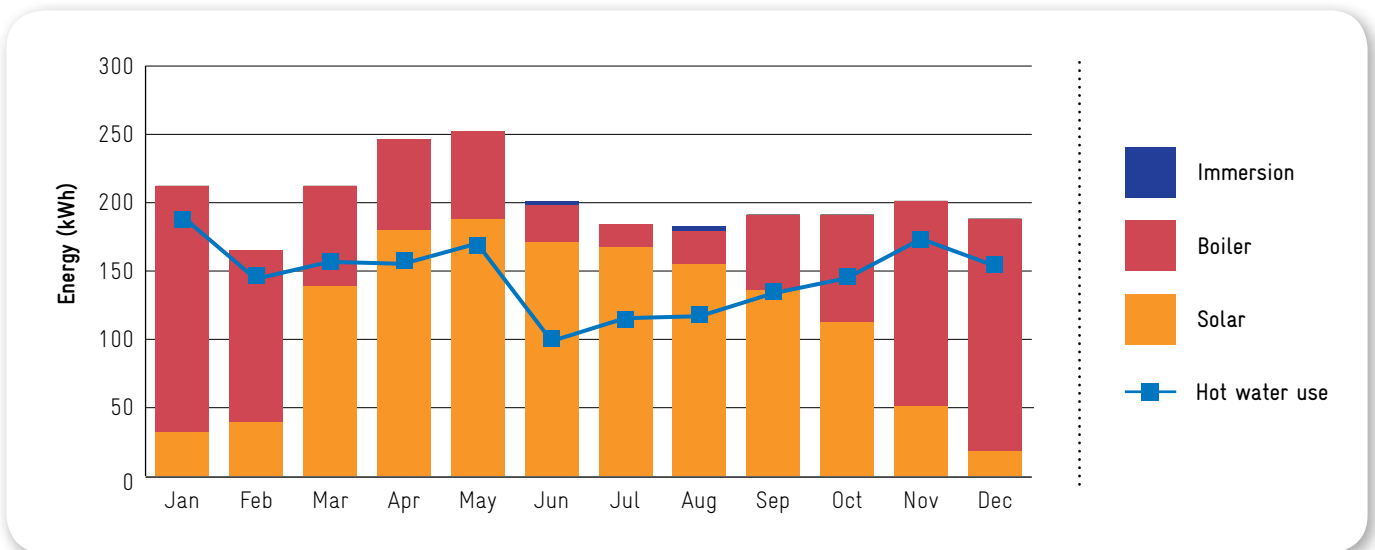
Figure 9. Graph showing a typical energy profile for a well-installed and properly run solar water heating system. The solar energy input to the hot water cylinder is at a maximum in summer, with back-up heating providing more energy in the winter months.
