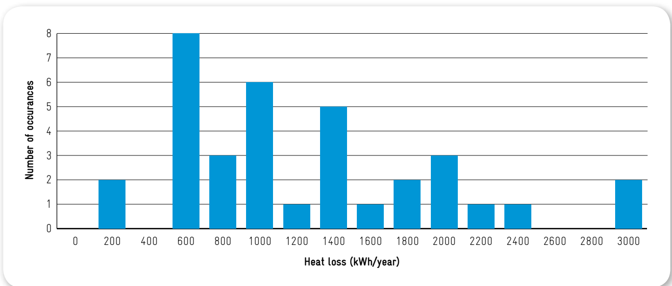
Figure 12. Heat loss from hot water storage cylinder
