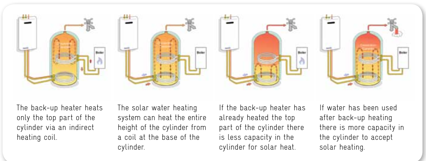
Figure 4. How a Twin-Coil Cylinder Works
